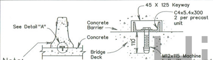
ELEVATION VIEW
