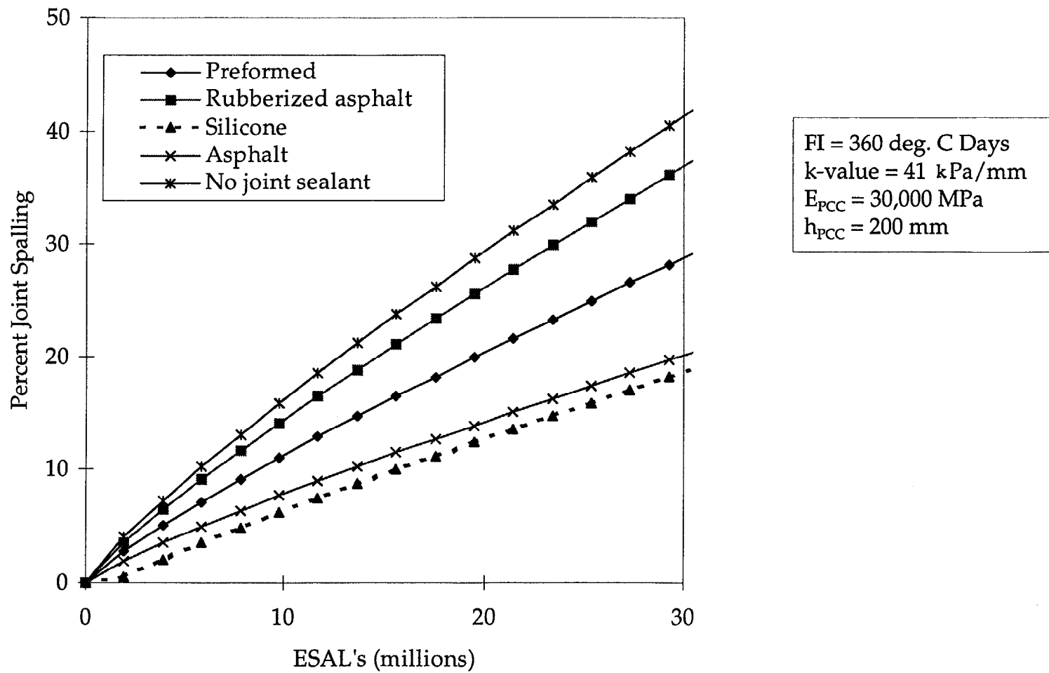
Figure 25. Influence of joint sealant type on JRC transverse joint spalling.
