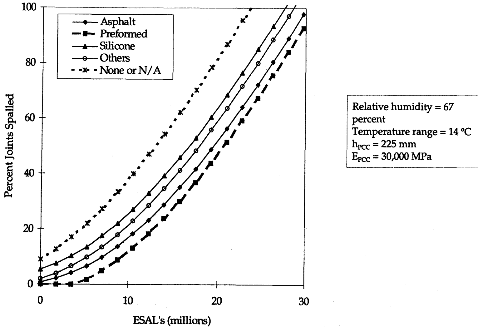
Figure 20. Plot of percent JPCP spalling versus traffic for the different joint sealant materials evaluated.
