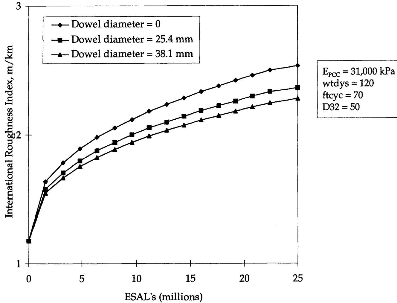
Figure 4. Plot of roughness versus traffic loadings, showing the effect of different dowel diameters.
