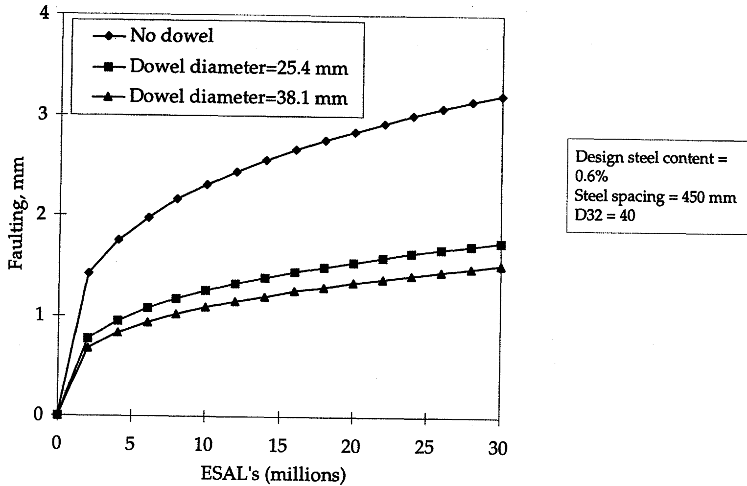
Figure 17. Influence of dowels on JPCP faulting.
