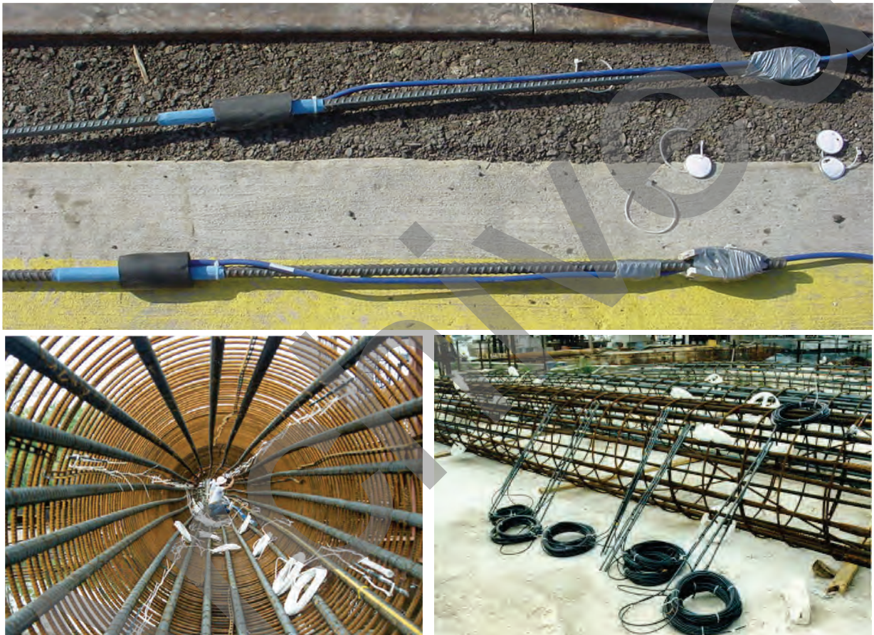
Figure 17-48 Sister-bar Mounted Strain Gauges Placed in Drilled Shaft Reinforcement
