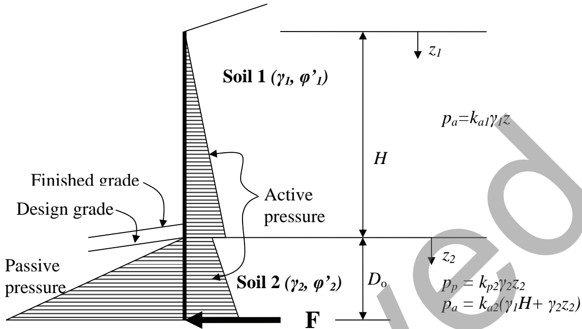
Figure 12-41 Simplified Earth Support Diagram for a Cantilever Wall using Effective Stress Strength
