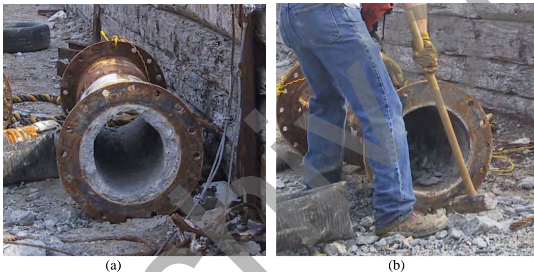
Figure 9-7 Tremie Must be Clean; (a) Tremie Contaminated with Hardened Concrete; (b) Worker Cleaning Tremie
