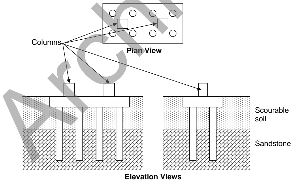
Figure 12-3 Example of a Drilled Shaft Group Foundation for a Bridge
