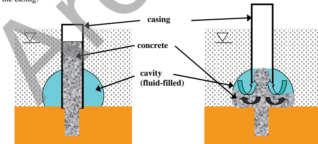
Figure 4-12 Breach of Casing/Concrete Seal During Casing Extraction Due to Cavity
