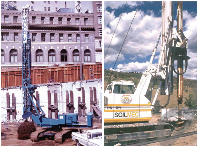
Figure 5-3 Mechanical (left) and Hydraulic (right) Powered Drilling Machines
