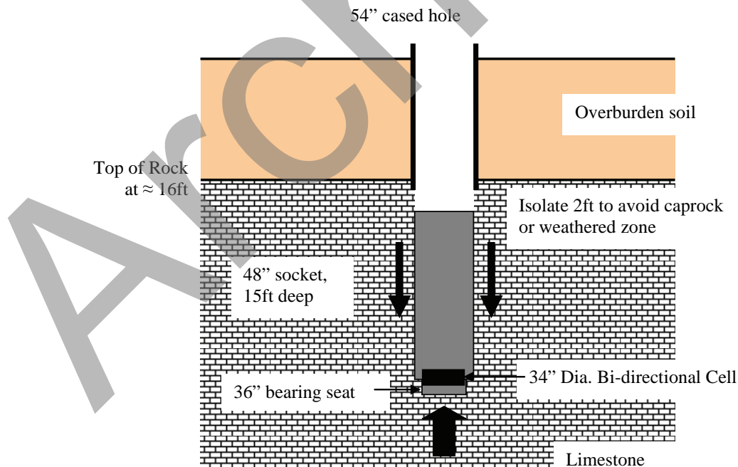
Figure 17-8 “Chicago Method” Load Test using Bi-directional Cell
