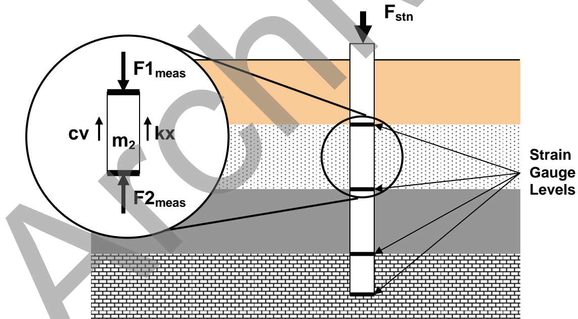
Figure 17-33 Segmental Unloading Point Method
