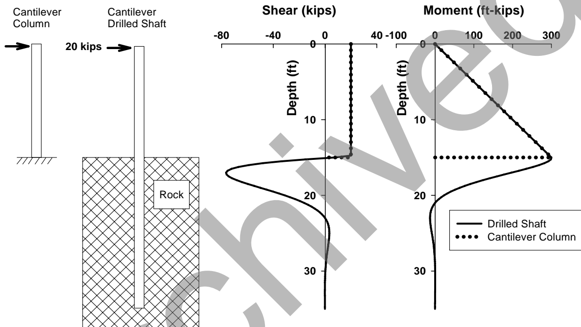
Figure 16-9 Comparison of Moment and Shear for a Cantilevered Column and a Docketed Drilled Shaft
