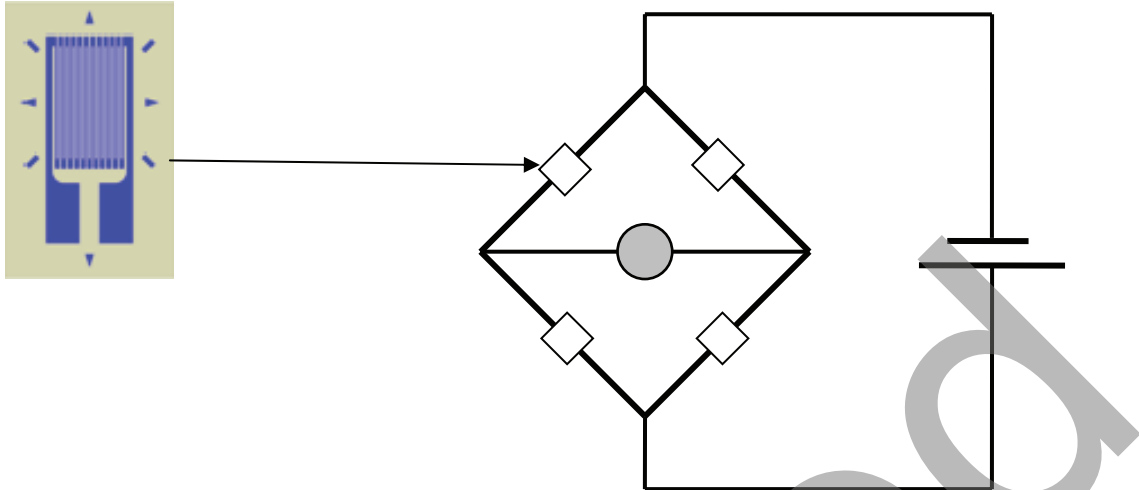
Figure 17-49 Resistance Type Strain Gauge
