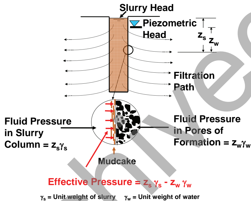
Figure 7-1 Formation of Filter Cake and Positive Effective Pressure, Mineral Slurry in Sand Formation
