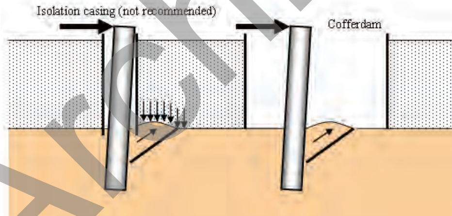
Figure 17-55 Schematic Diagram of Lateral Test where Scourable Overburden is Present
