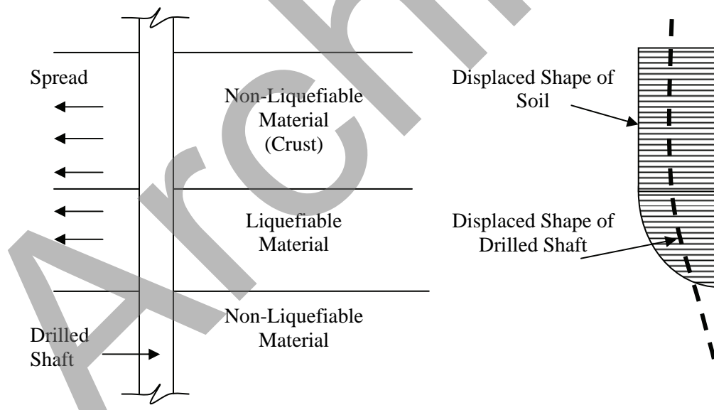
Figure 12-45 Spreading that Displaces Foundation with Soil
