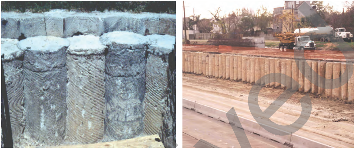
Figure 1-18 Drilled Shaft Secant Wall (left) and Tangent Wall (right)
