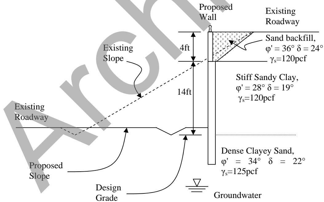
Figure 12-42 Example of Drilled Shaft Wall Problem
