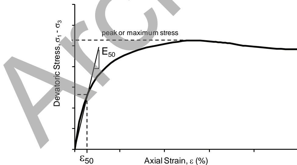
Figure 3-7 Example of Soil Stress-Strain Curve and 50% Secant Modulus
