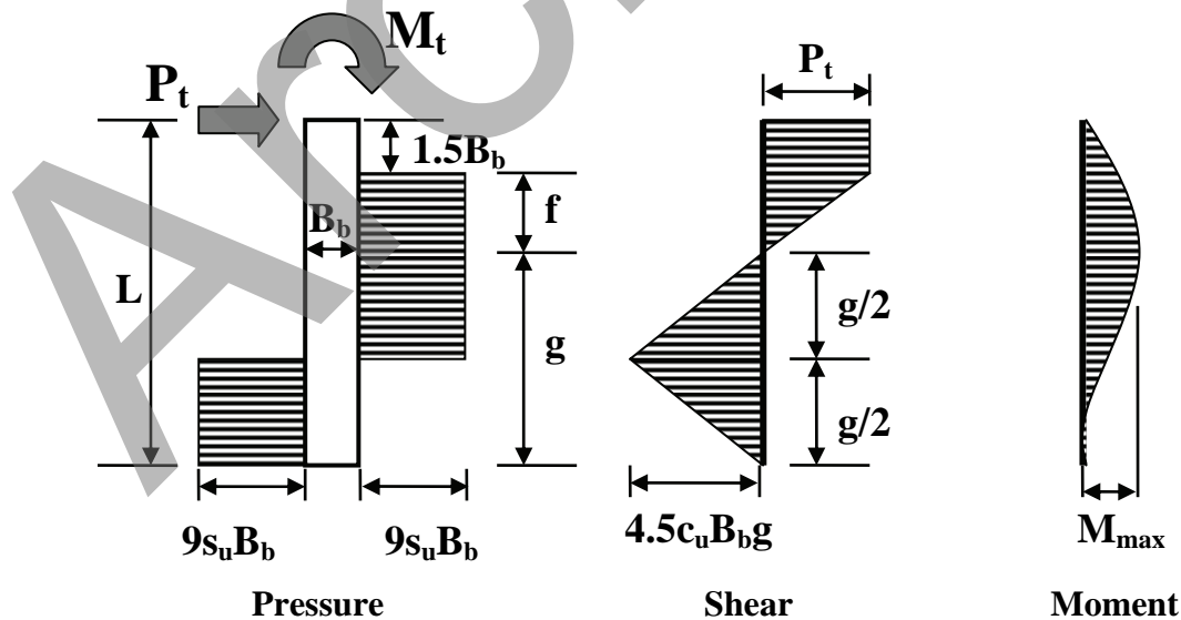
Figure 12-37 Broms Pressure, Shear, Moment Diagrams for Cohesive Soils
