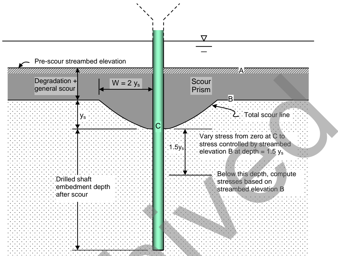
Figure 13-18 Illustration of Scour Prism and Effects on Drilled Shaft
