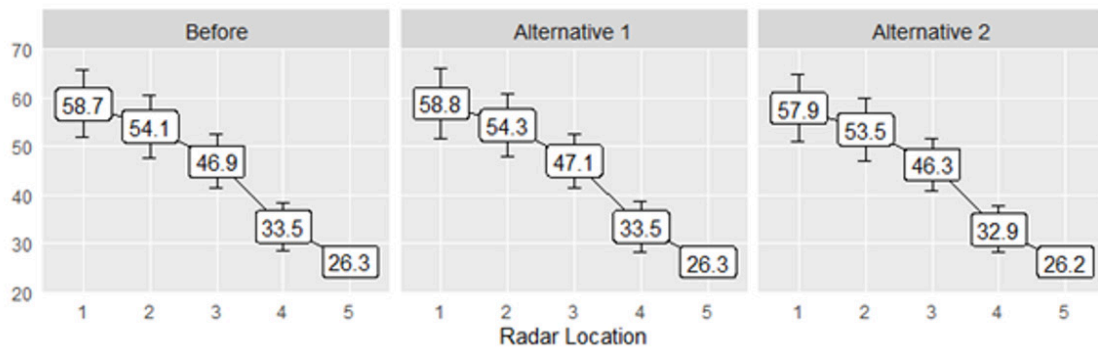
Figure 22. Graphs. Speed profiles, MD-3: mean speed (mph) \pm 1 standard deviation by radar location and alternative.
