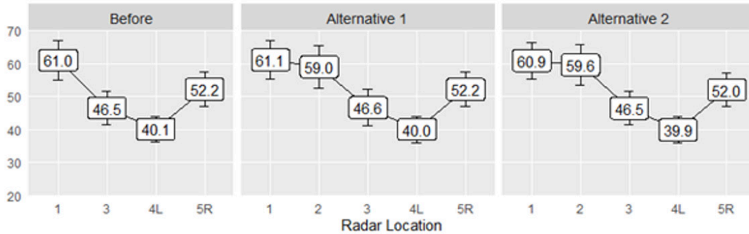
Figure 20. Graphs. Speed profiles, MD-1: Mean speed (mph) \pm 1 standard deviation by radar location and alternative.
