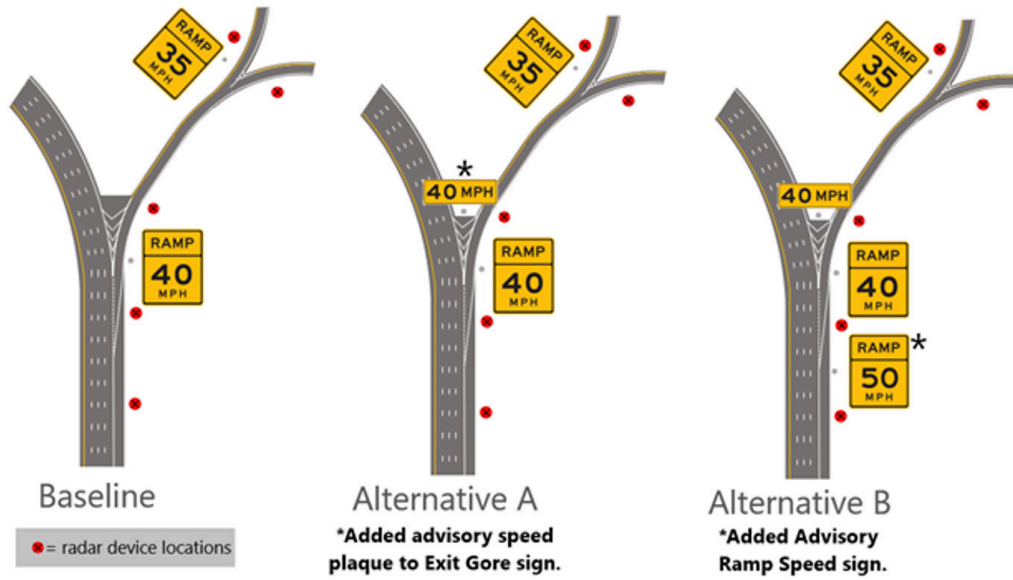
Figure 14. Illustration. Signing treatments for MD-2 site.
