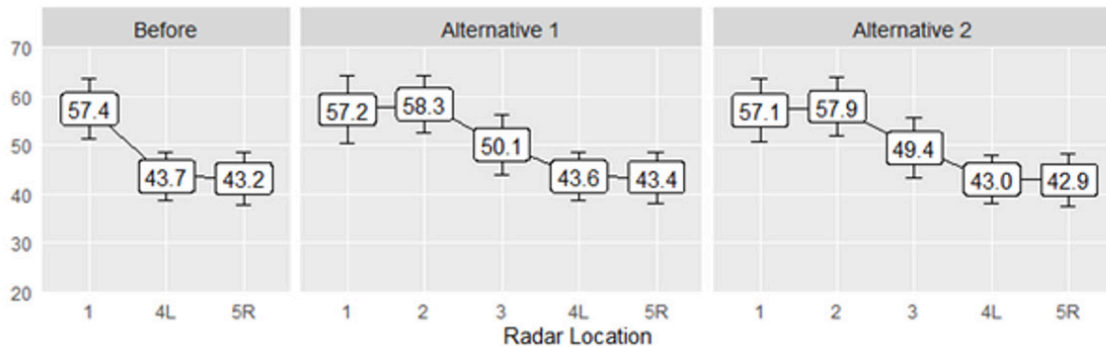
Figure 21. Graphs. Speed profiles, MD-2: mean speed (mph) \pm 1 standard deviation by radar location and alternative.
