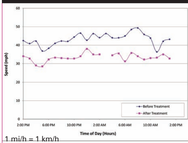
Figure 24. "Before-After" average speeds for southbound approach on minor road.
