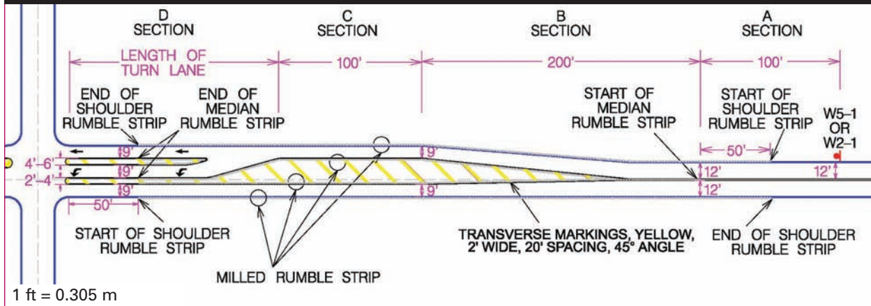
Figure 16. Typical design of concept 1 with left-turn lanes.
