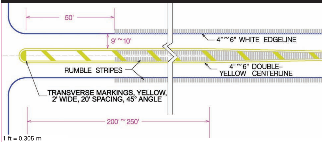
Figure 26. Illustration of enhancements to section C of concept 1 with rumble strips.
