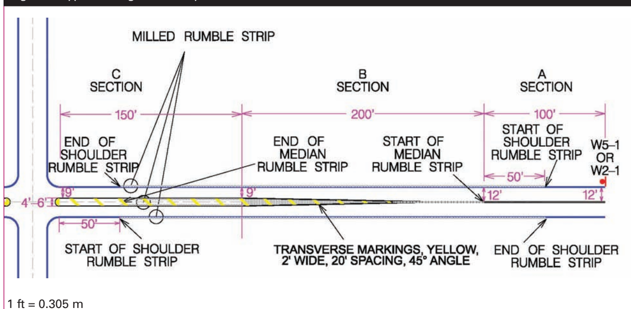
Figure 6. Typical design of concept 1.
