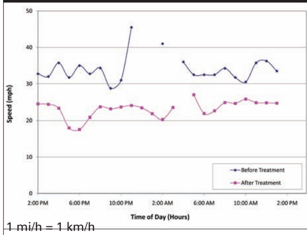
Figure 23. "Before-After" average speeds for northbound approach on minor road.
