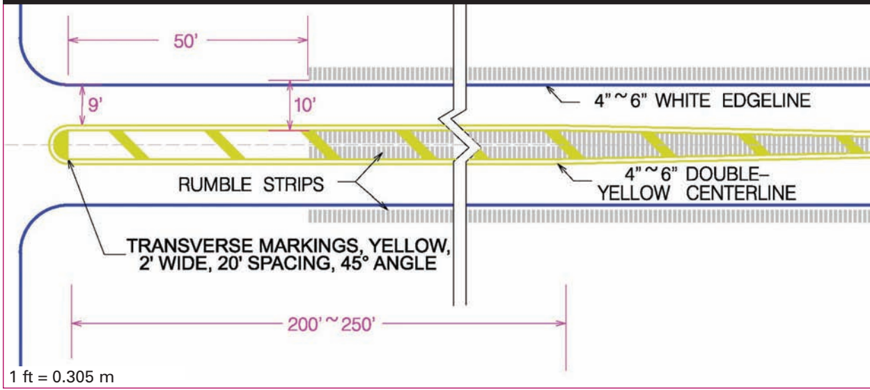
Figure 25. Illustration of enhancements to section C of concept 1 with rumble strips.
