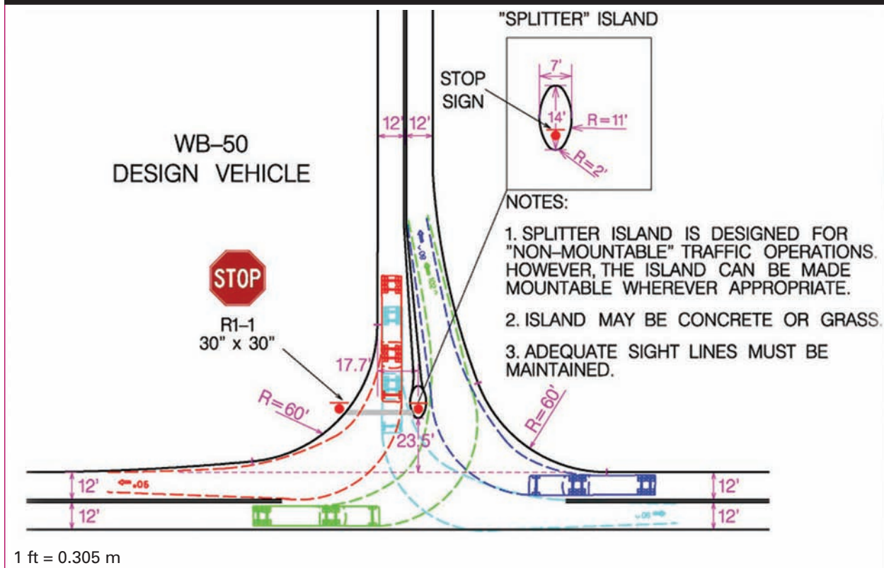
Figure 8. Typical design of concept 2.
