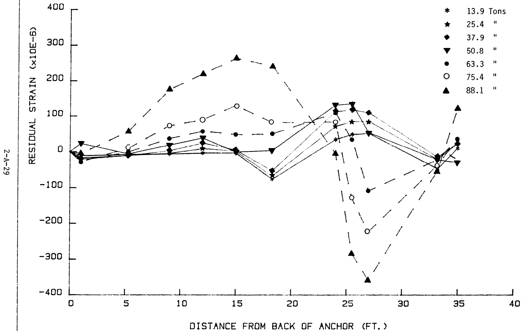
Figure 29. Distribution of Residual Strain in the Deformed Metal Tube of Tieback 18-2.
