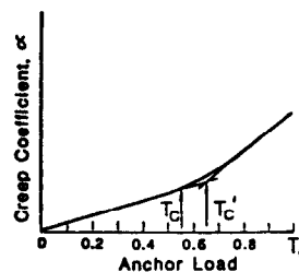
B. CREEP COEFFICIENT PLOT
