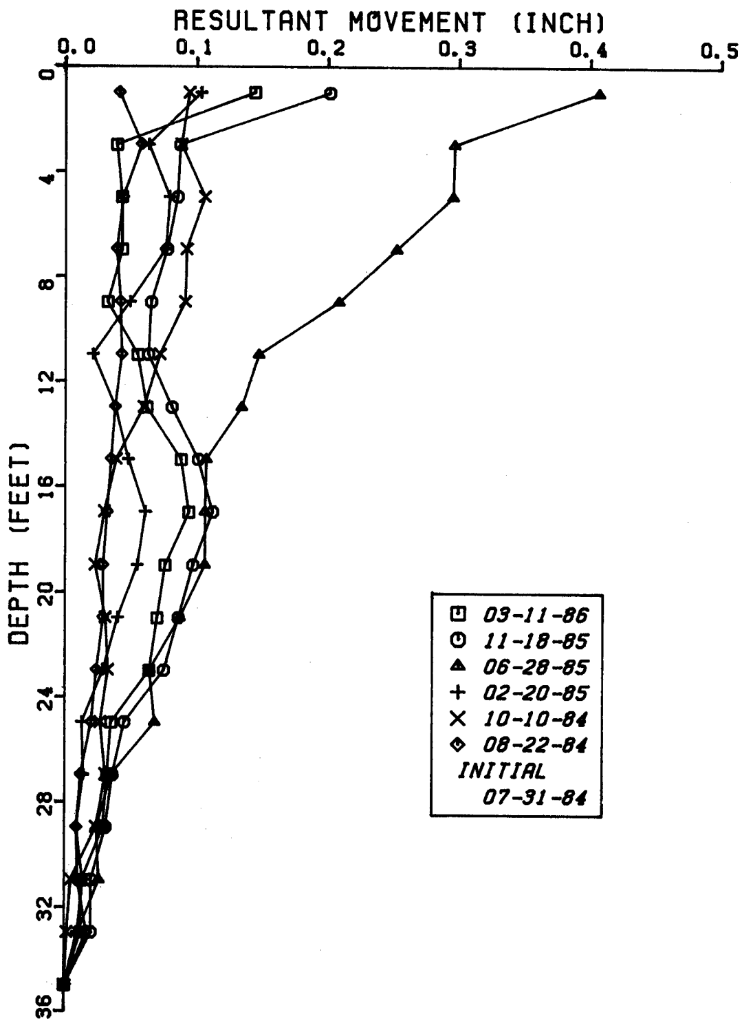
FIGURE 24. SLOPE INCLINOMETER 11 - LATERAL MOVEMENT AT STATION 236 + 00, 85 FEET RIGHT.
