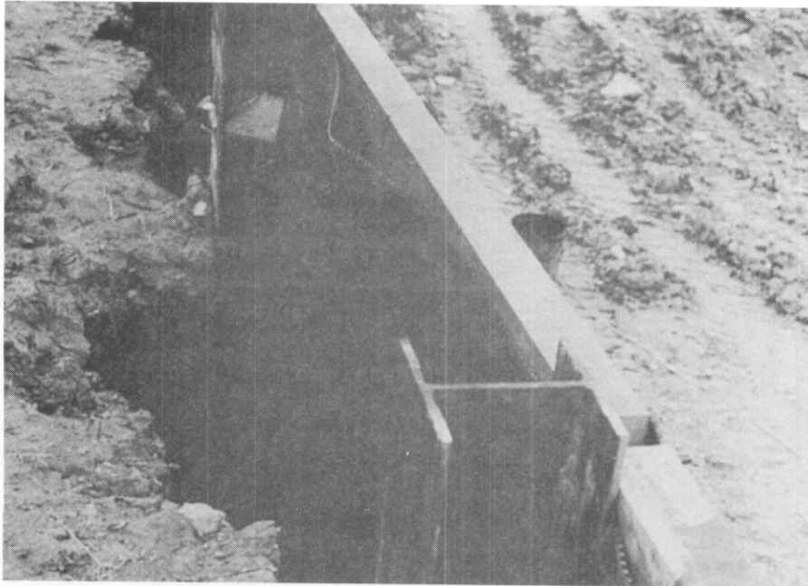
Figure 10. Drainage Pathway of AMOCO 4553 Fabric against The Earth and TENSAR "PWI" Grid against The Lagging.
