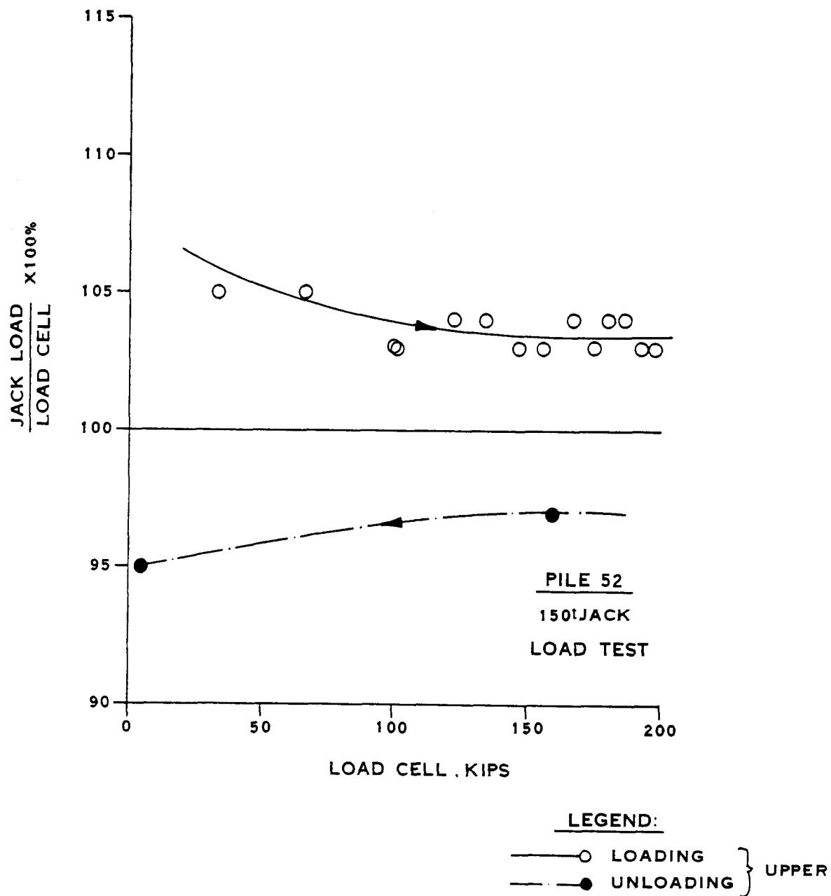
FIGURE 27 COMPARISON OF LOAD CELL AND HYDRAULIC JACK DURING LOAD TEST
