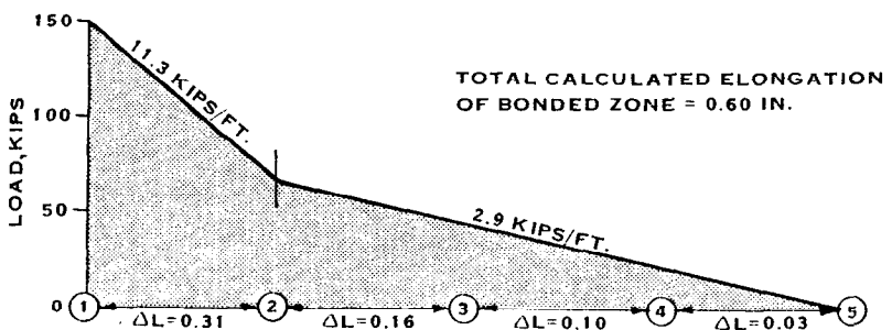
A. HYPOTHETICAL LOAD TRANSFER DIAGRAMS WITH CALCULATED TOTAL BONDED ZONE ELONGATION = 0.60 INCH
