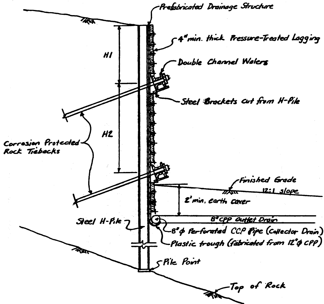
Figure 6. Typical Tieback Wall Section.
