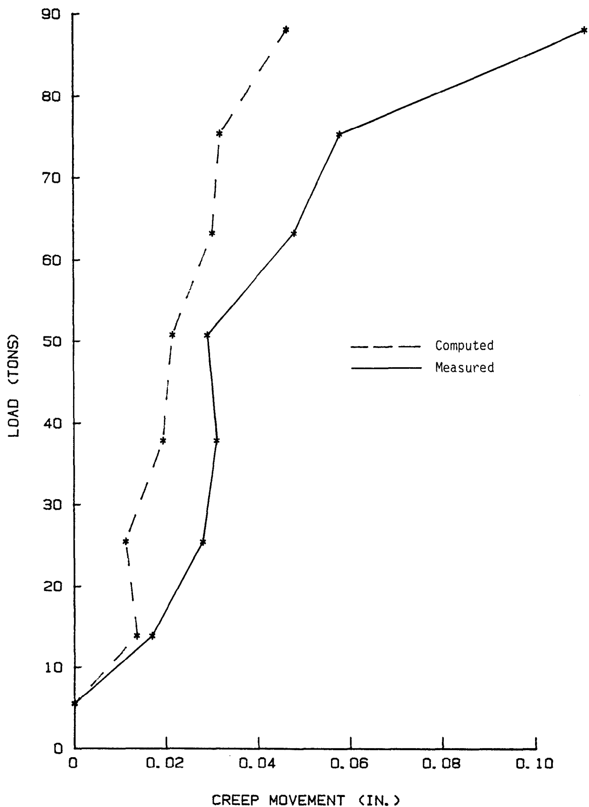
Figure 21. Measured Versus Computed Creep Movement of Tieback 15-8
