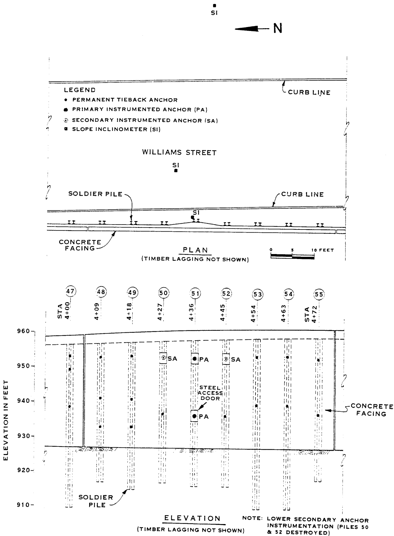
FIGURE 2 - PERMANENT TIEBACK WALL INSTRUMENTATION
