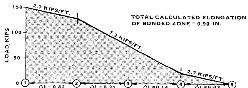
B. HYPOTHETICAL LOAD TRANSFER DIAGRAMS WITH CALCULATED TOTAL BONDED ZONE ELONGATION = 0.90 INCH
