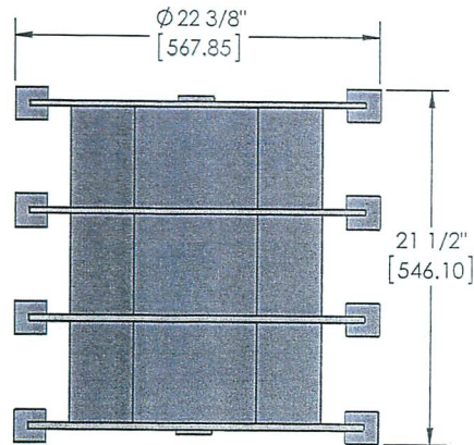
SLED END TREATMENT TRANSITION FRAME
