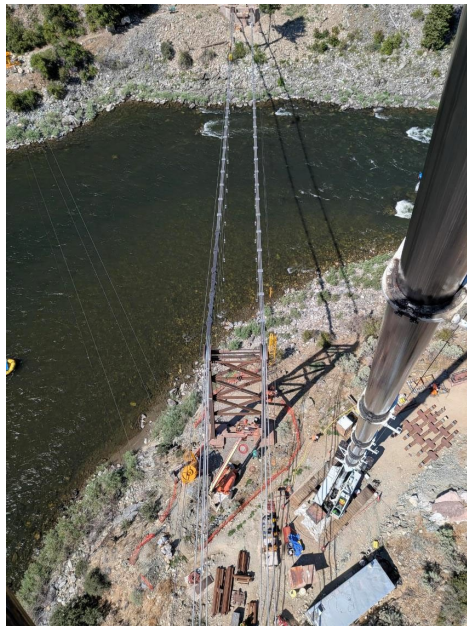
Overhead view of cable system.
