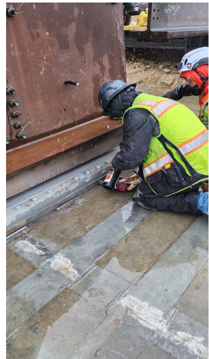
Mag Particle Testing Bering Welds
