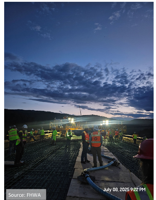
Start of First Deck Pour.
