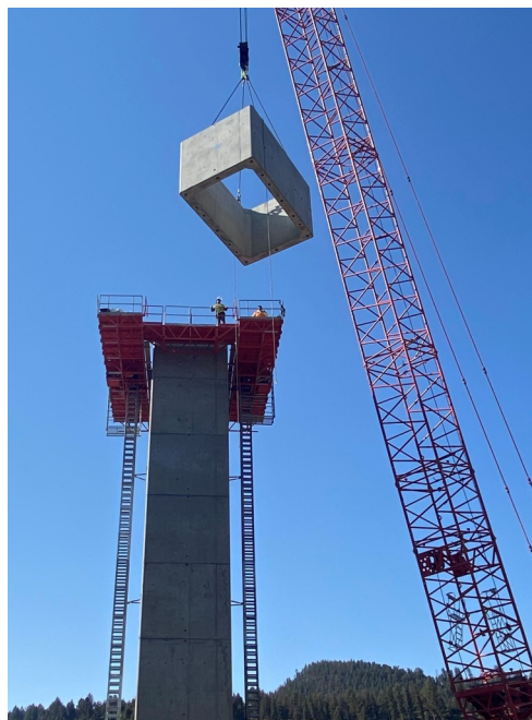
Stacking Pier 2
