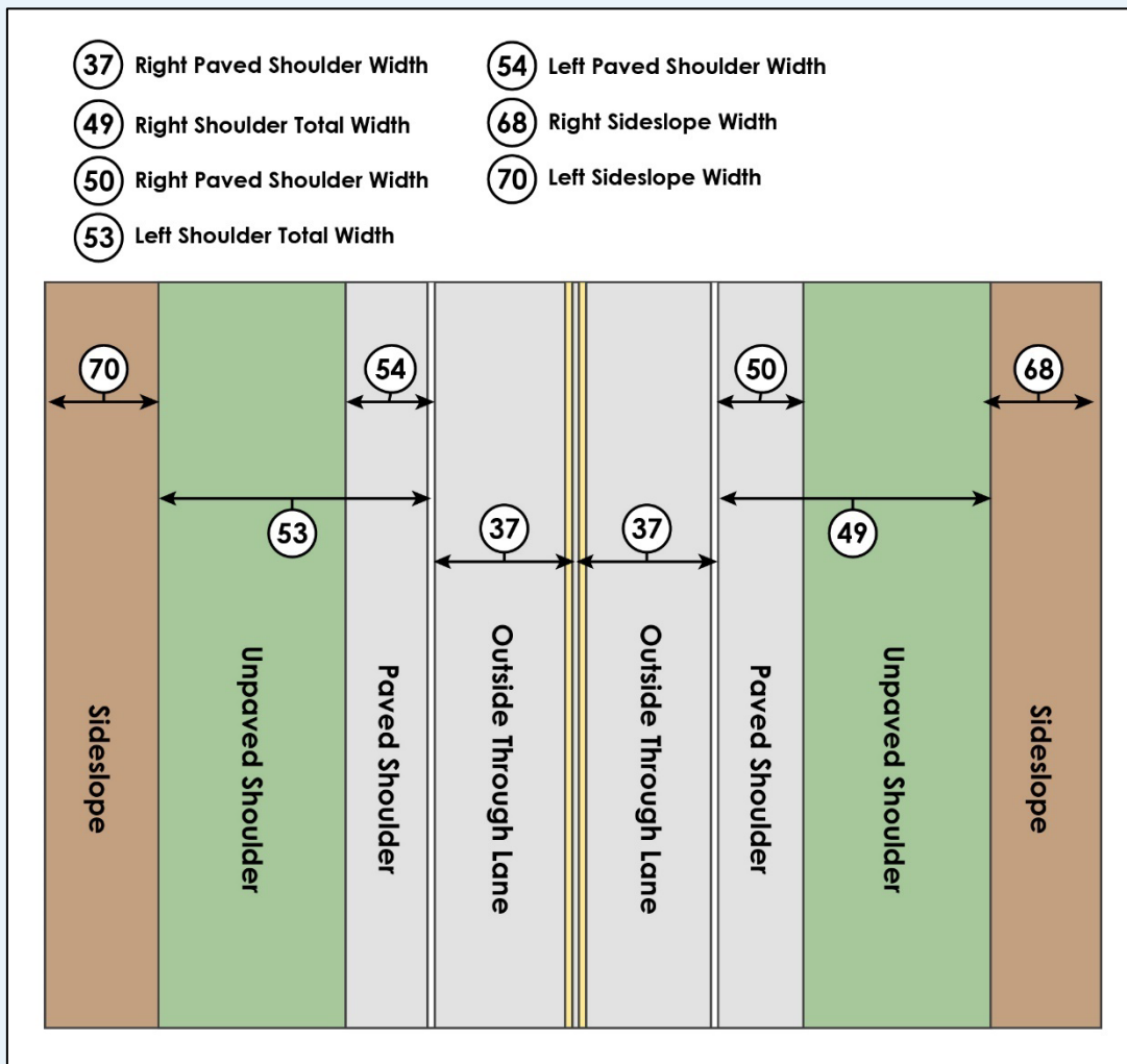
Figure 15. Graphic. Illustration of cross section, two-lane roadway.
