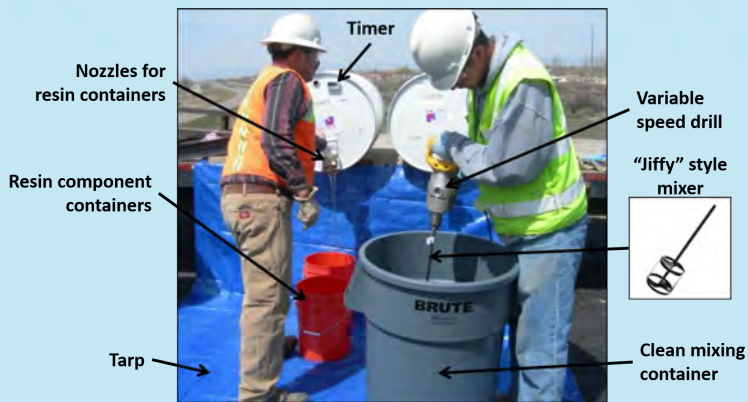
Figure 11. Photograph. Typical tools and equipment for resin binder proportioning and mixing for manual application.
