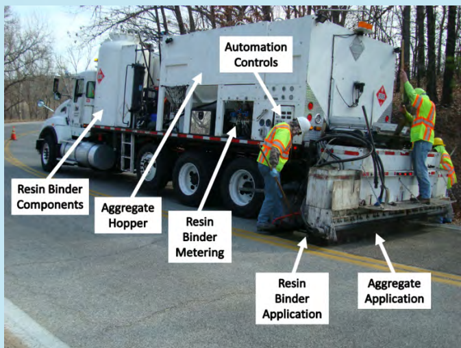
Figure 16. Photograph. Example of a fully-automated installation vehicle.
