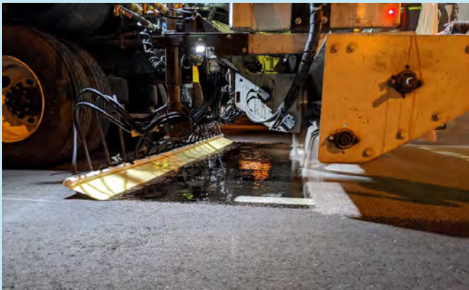
Figure 18. Photograph. Example of fully automated resin binder application followed by automated aggregate application demonstrating uniformity of coverage.
