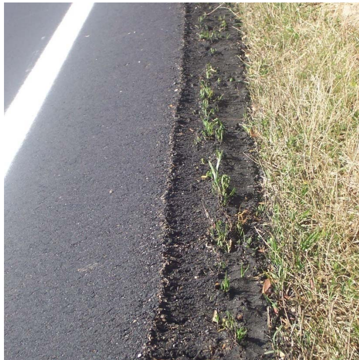
Figure 6. Example of Safety Edge SM placed on heavy vegetation – due to lack of adequate compaction the Safety Edge SM will deteriorate.
