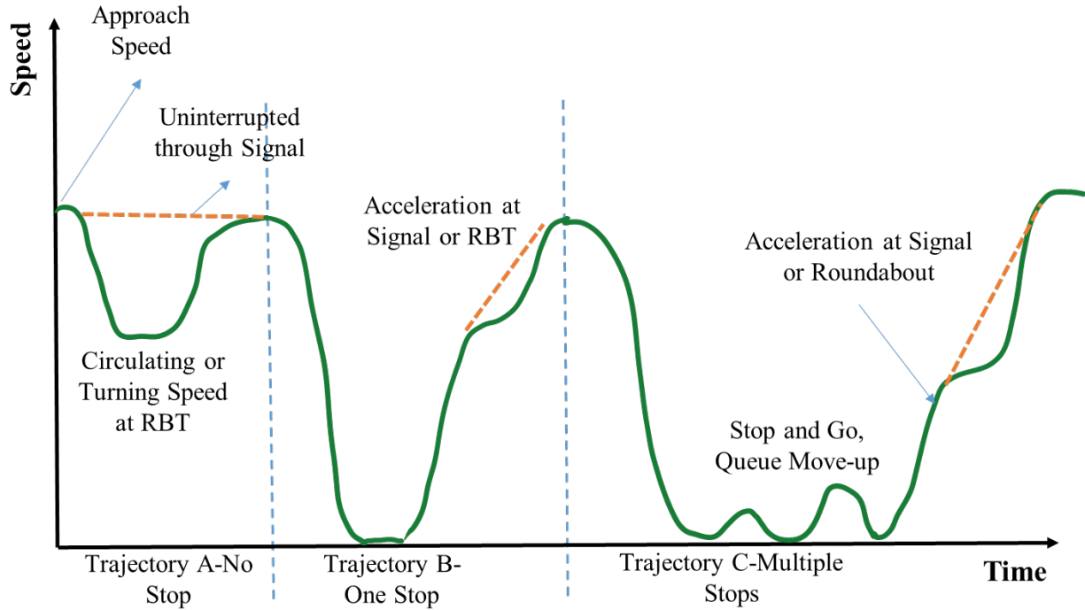
Figure 5. Graph. Illustration of the three types of trajectories (A: no-stop, B: one-stop, and C: multiple-stops) for a roundabout and signalized intersection approach.
