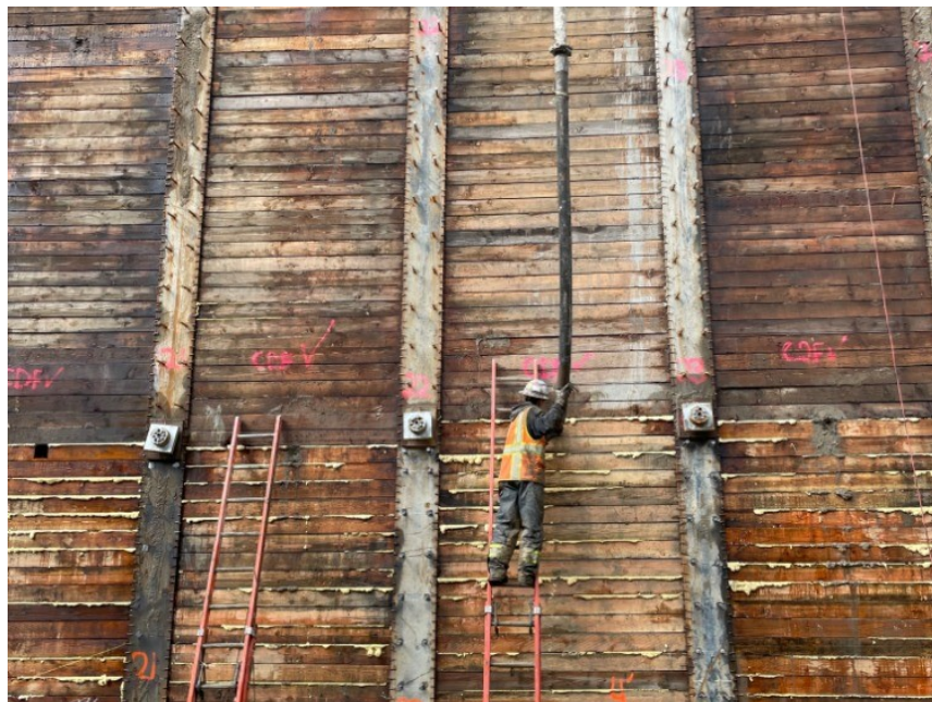
Photo left: Shows Placing Slurry behind timber lagging. at MP 56. All images Source: FHWA
