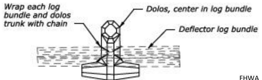
Typical drawing of the assembled Dolos-Log Bundles
