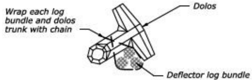
Log bundles will be chained to these concrete dolos and the assembled units will be used to create the Engineered Log Jams
