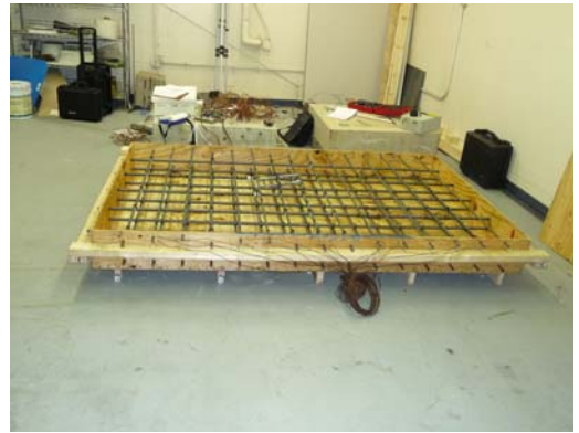
Figure 6. Photo. Bridge deck specimen with reinforcing bars.
