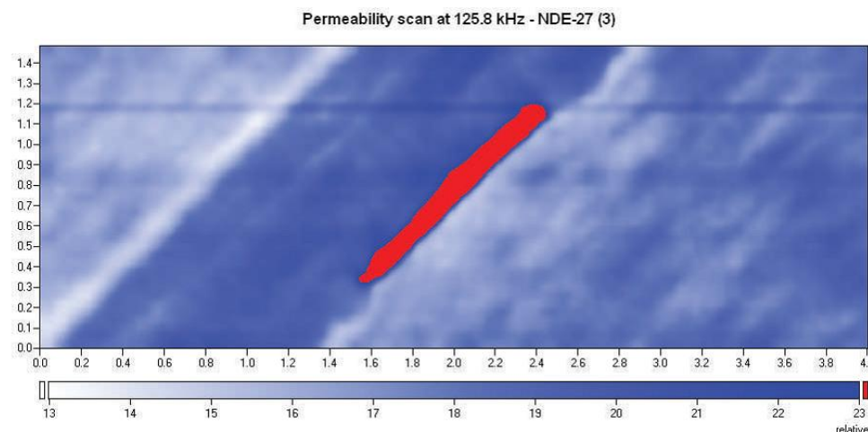
Figure 4. Graph. Permeability C-scan image using an FA28 MWM Sensor oriented 45 degrees with respect to weld on butt-weld specimen with a surface flaw of length 30.48 mm (1.2 inches). The defect is shown as a red line on the image.
