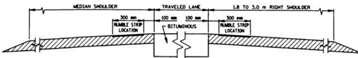
SECTION VIEW OF MULTI-LANE ROADWAY - Types 2 and 3 (ONE ROADWAY SHOWN)
