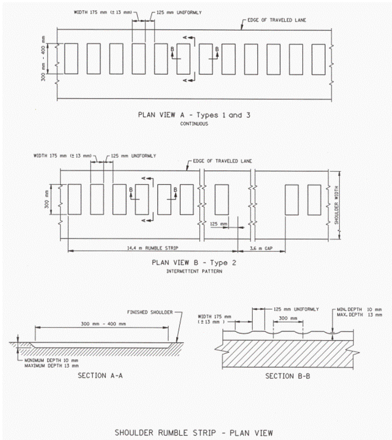
Figure 2.1.1. Shoulder Rumble Strip - Plan View (Metric).
