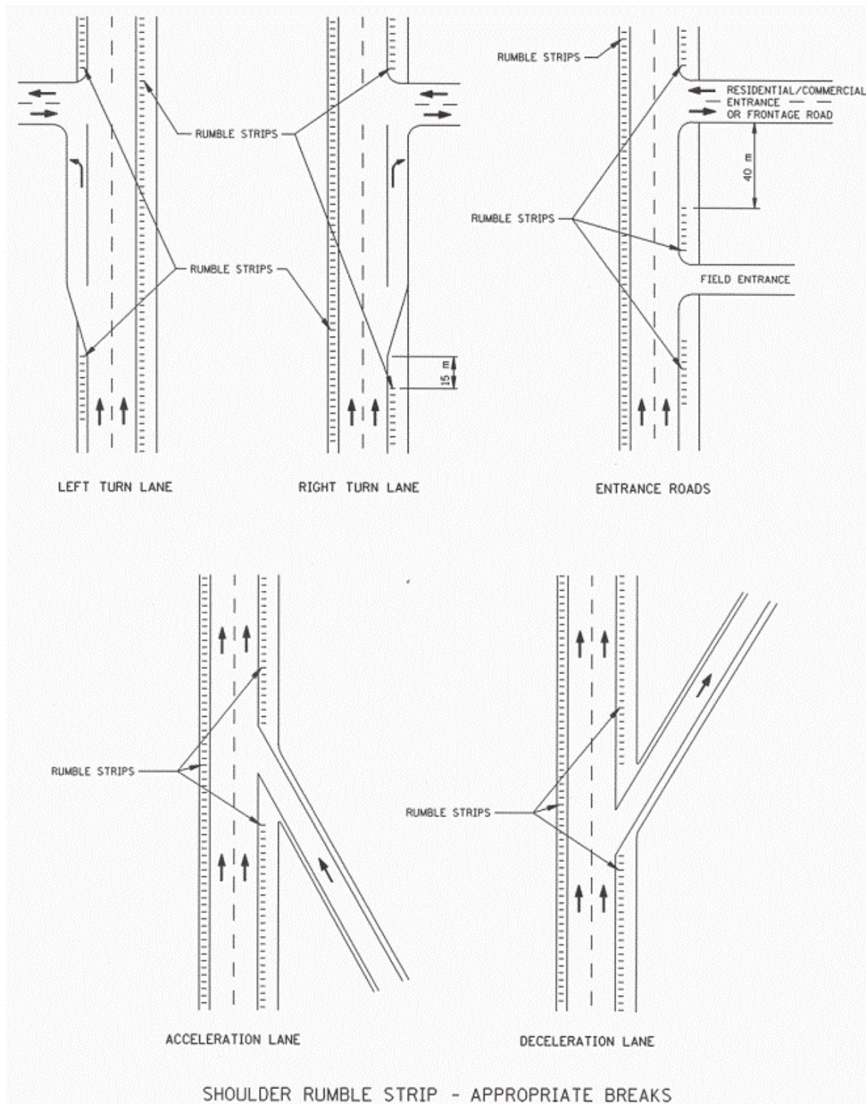
Figure 4.1.1. Shoulder Rumble Strip - Appropriate Breaks (Metric).
