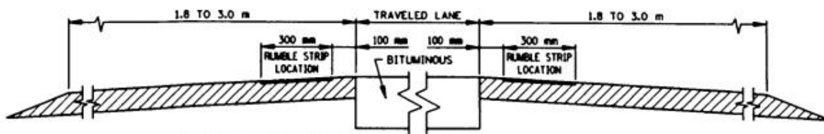
SECTION VIEW OF TWO-LANE ROADWAY - Types 2 or 3 (WITH 1.8 TO 3.0 m PAVED SHOULDERS)
