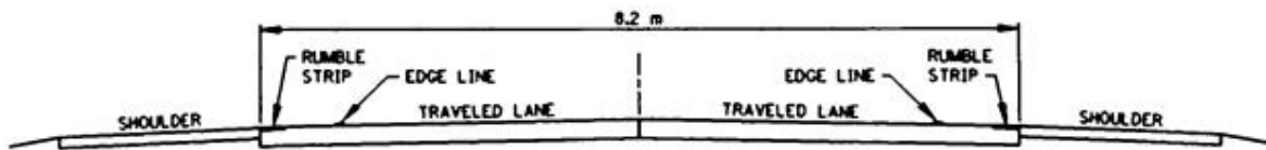
SECTION VIEW OF ROADWAY
