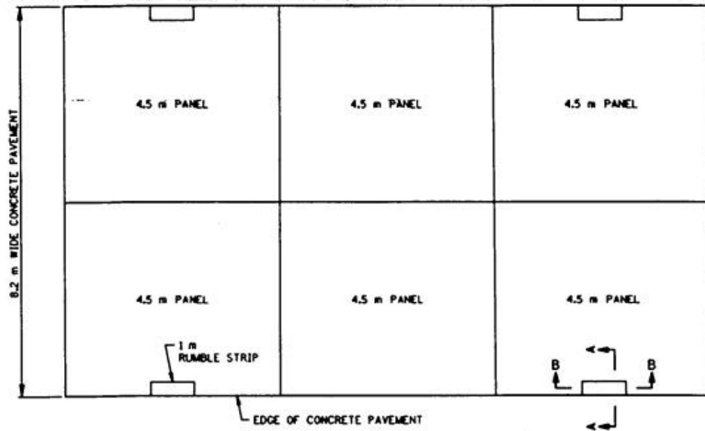
PLAN VIEW - Type 4
