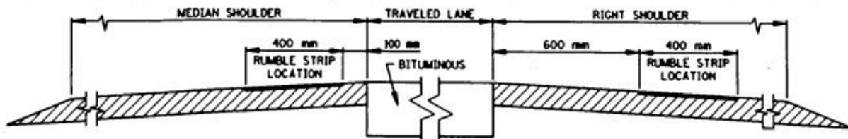
SECTION VIEW OF FREEWAY - Type 1 (ONE ROADWAY SHOWN)
