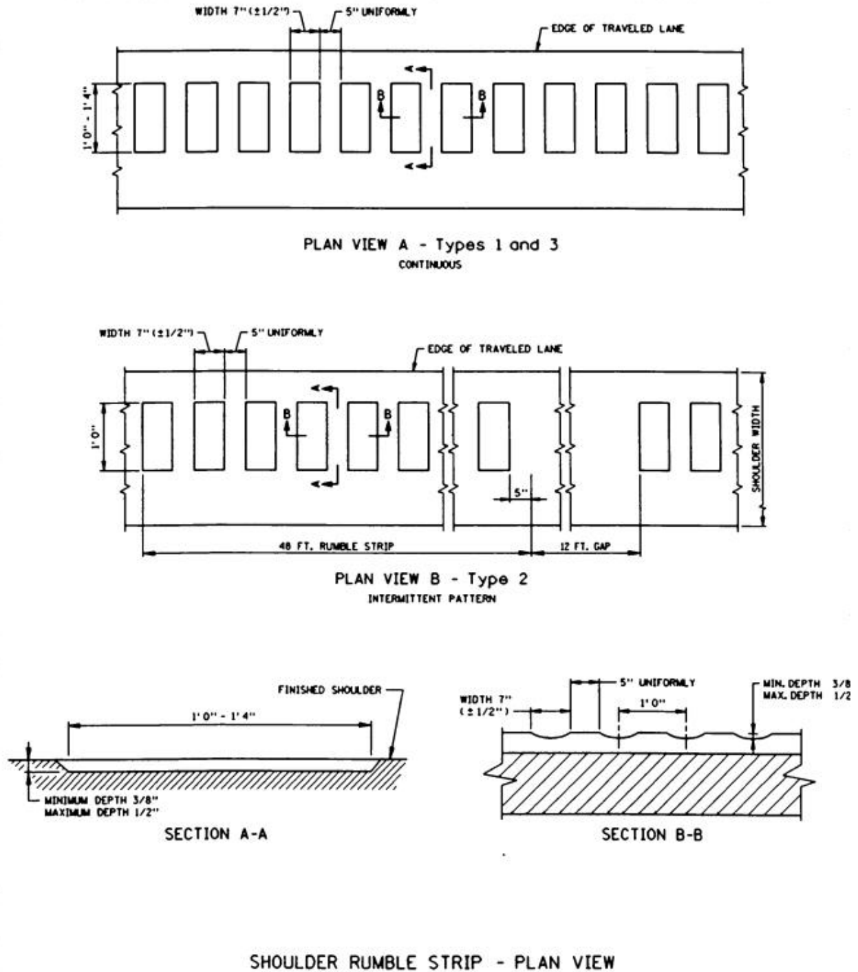
Figure 2.1. Shoulder Rumble Strip - Plan View (English).
