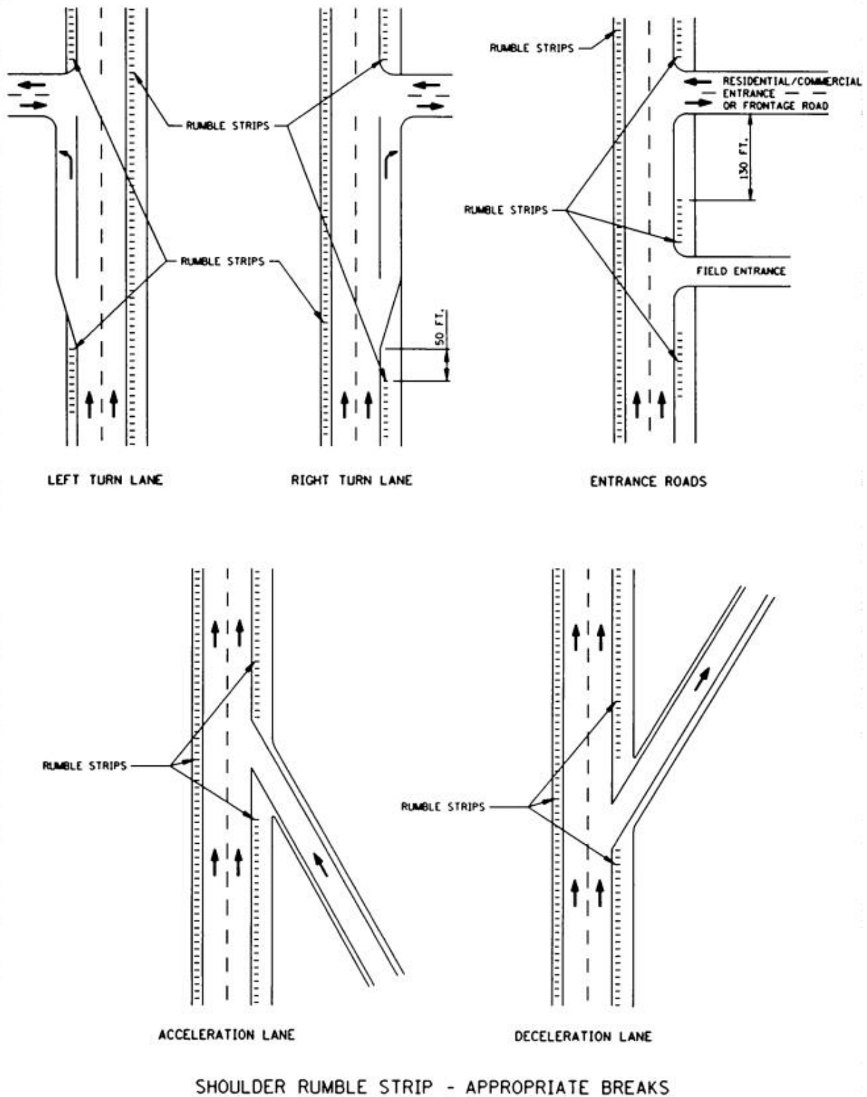
Figure 4.1. Shoulder Rumble Strip - Appropriate Breaks (English).
