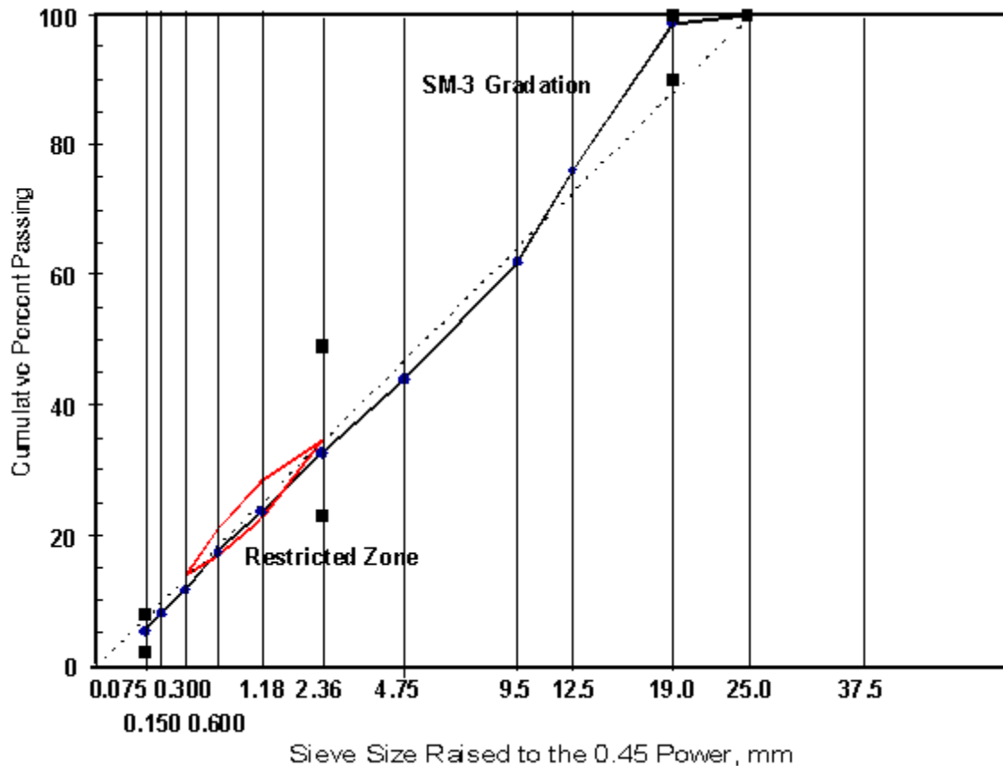
Figure 2. Aggregate gradation.
