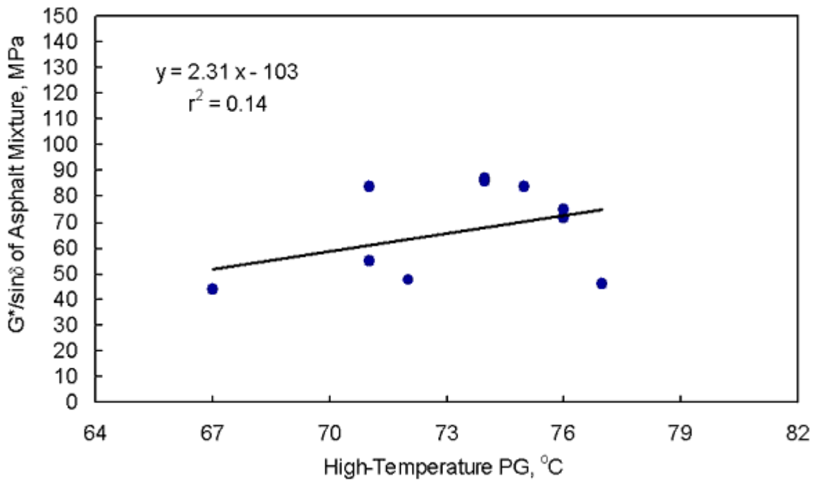
Figure 7. G^*/\sin\delta of the asphalt mixture at 50°C vs. high-temperature PG using the 11 asphalt binders.
