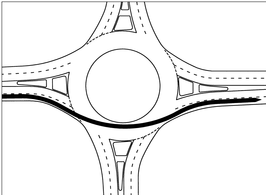
Exhibit 2-4. Fastest vehicle path through a double-lane roundabout.
