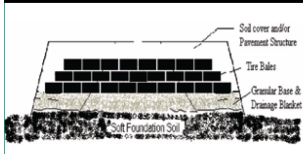
Figure 9. Application of tire bales.
