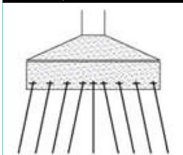
Figure 3. Hybrid shaft consisting of high-strength tendons or micropiles installed at the rock face.
