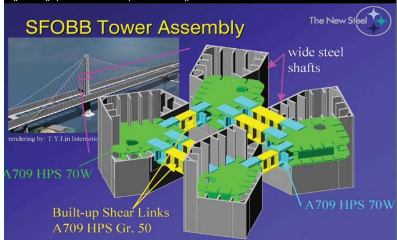
Figure 6. High-performance steel as permanent casing for drilled shaft foundations.
