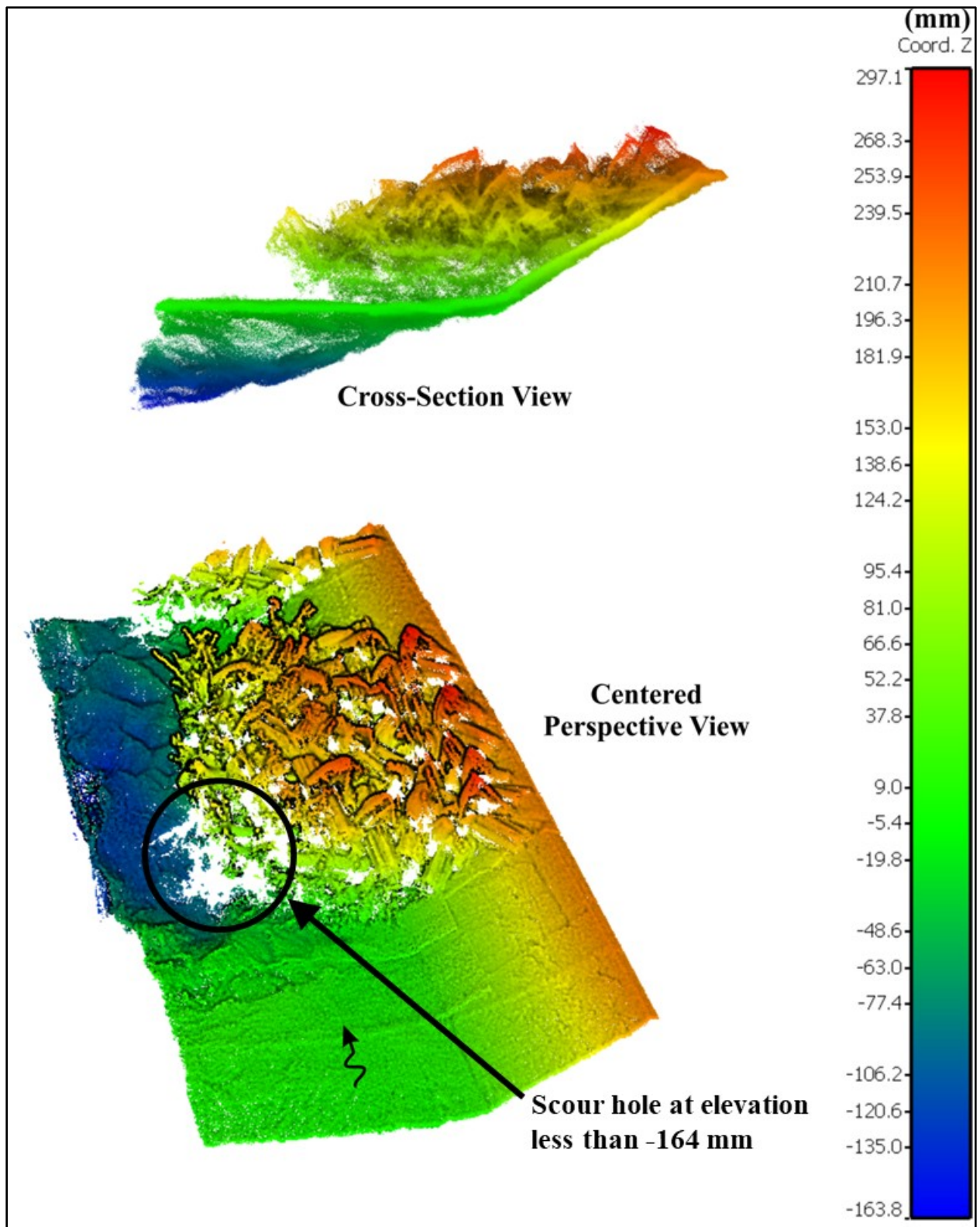
Figure 30. Graphic. Bathymetric map showing ELJ unit and scour for run I-2.
