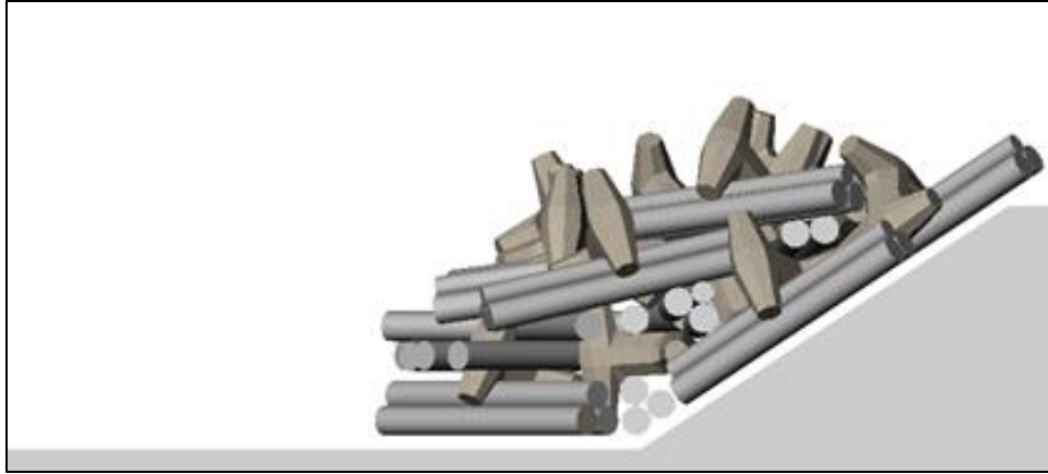
Figure 62. Graphic. Cross-sectional view of the CFD geometry of an ELJ unit.
