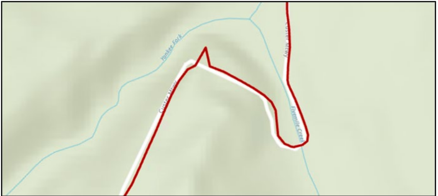
Figure 13. Graphic. Example of a harsh angle in centerline geometry.
