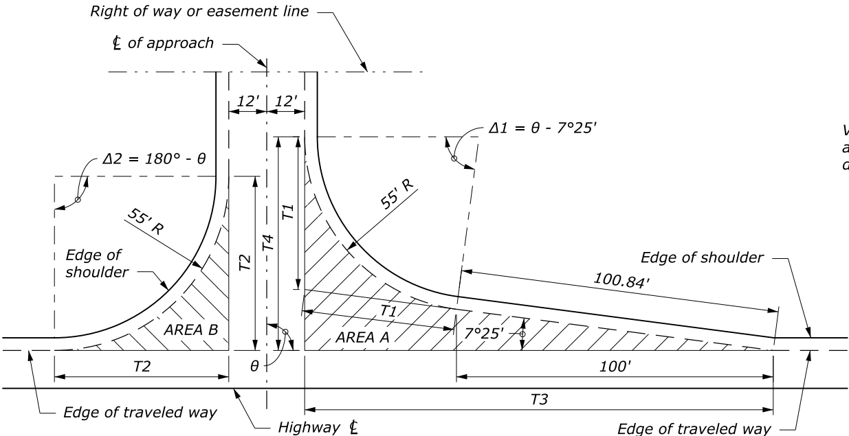
PLAN OF TYPE M APPROACH
