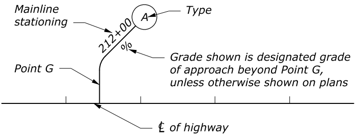
ROAD APPROACH LOCATIONS ON PLAN SHEETS
