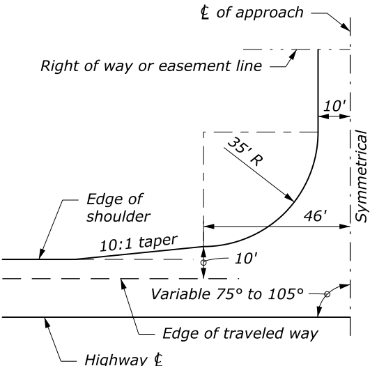
PLAN OF TYPE B APPROACH
