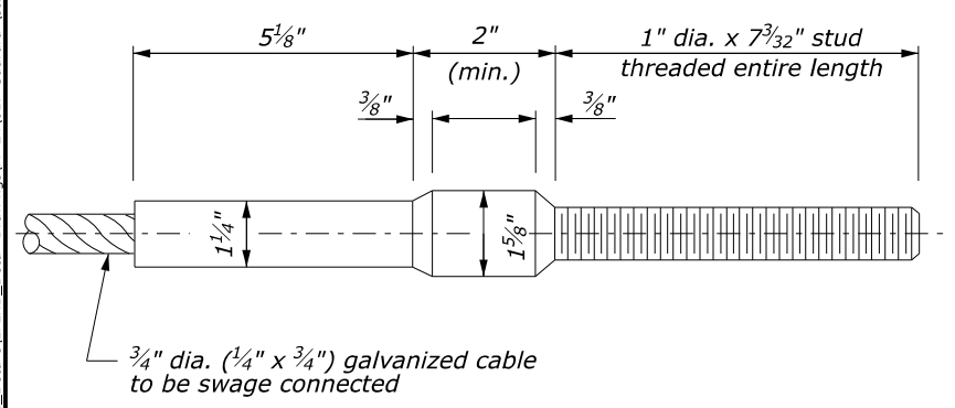
CABLE ANCHOR ASSEMBLY ARTBA F-37-76 (Standard swaged fitting and stud)
