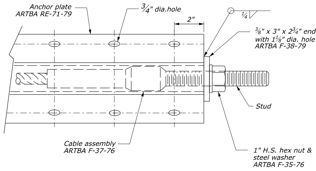
CABLE ANCHOR PLATE DETAILS ARTBA RE-71-79
