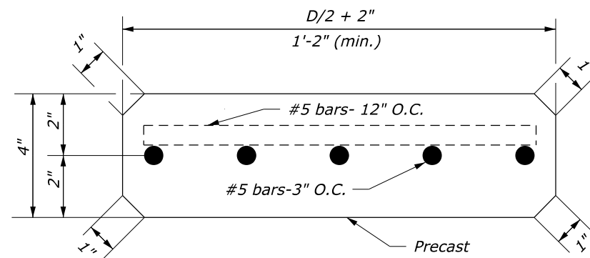
SLAB-B
