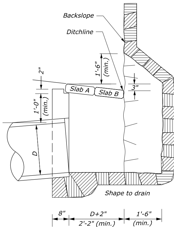
TYPE - 4C See Note 5
