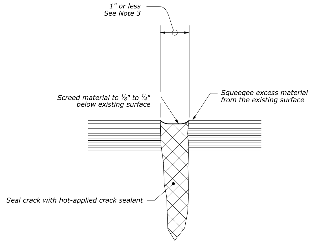
CRACK SEALING
