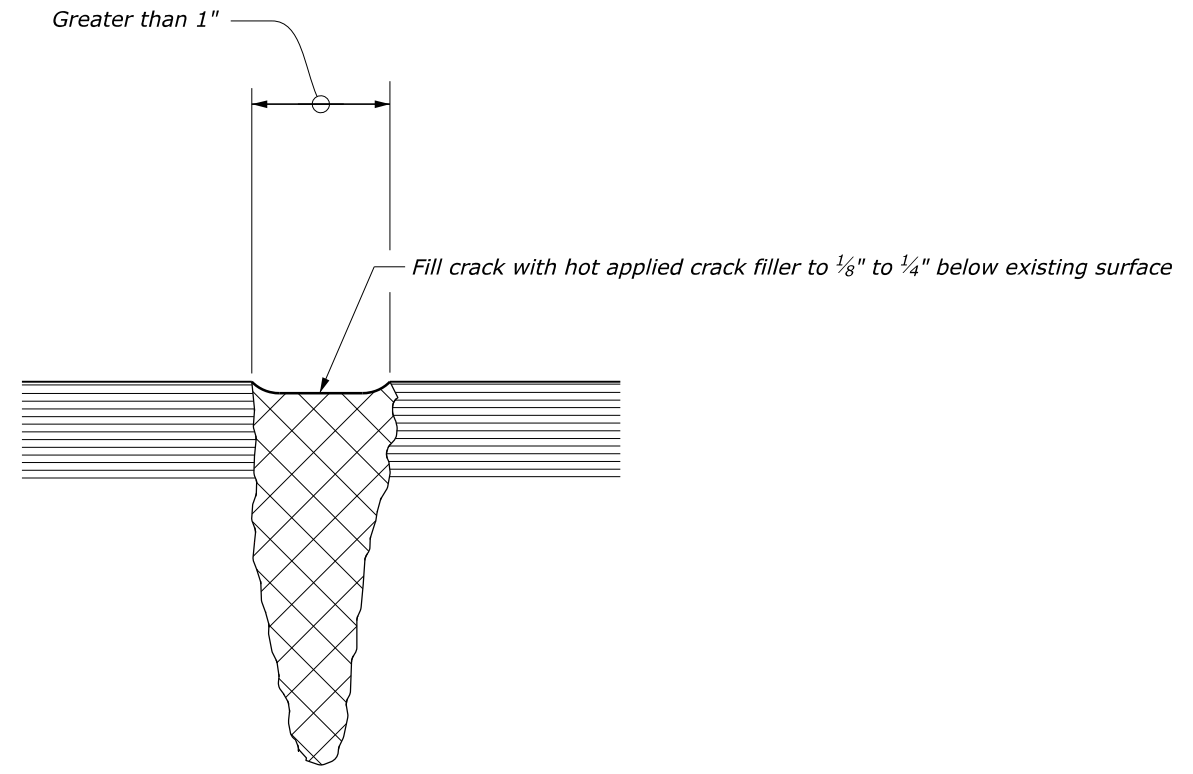
CRACK FILLING
